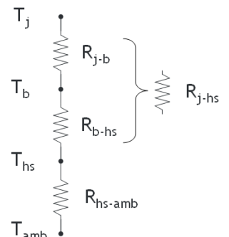
Figure 3: Series Thermal Resistance
